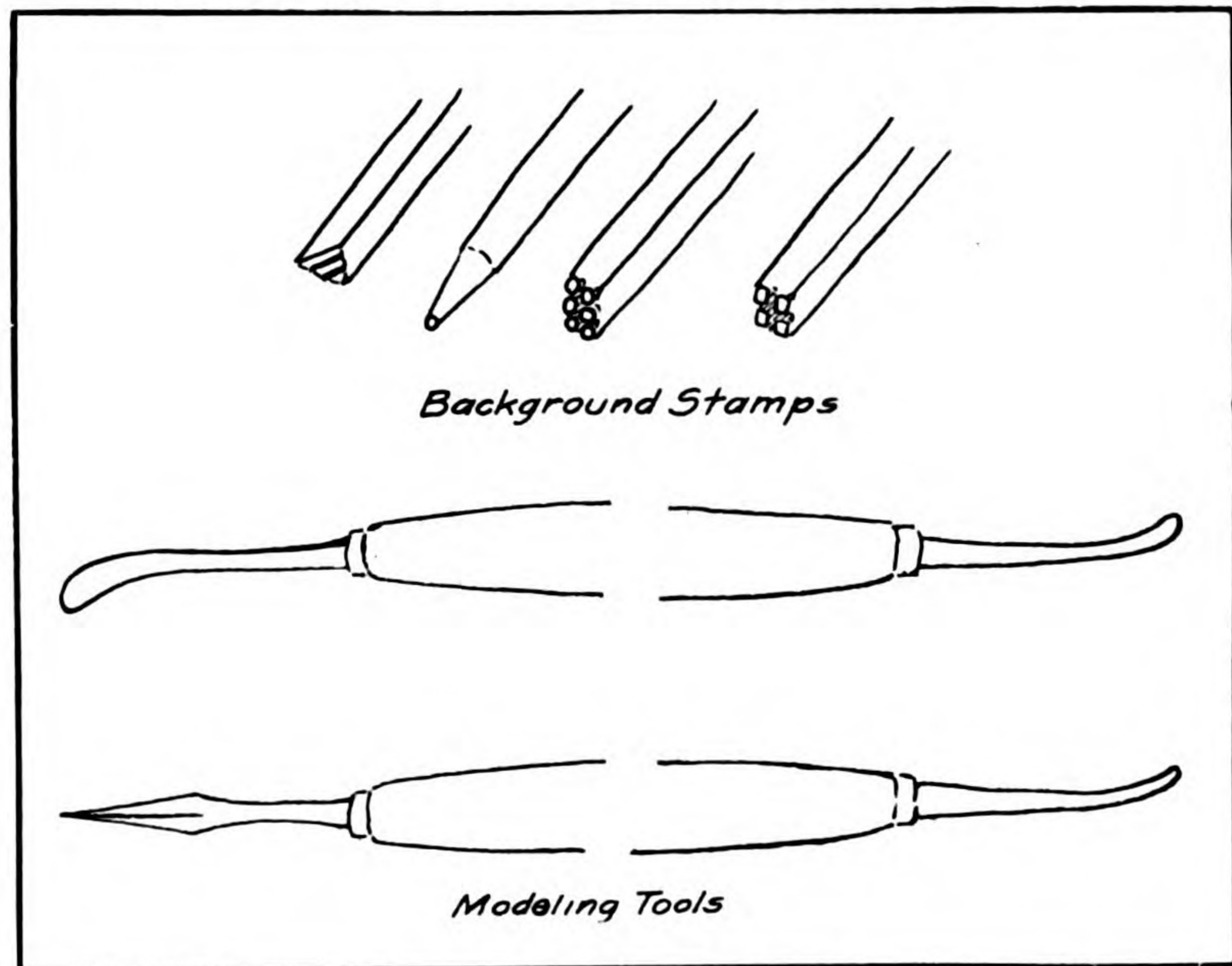
Fig. 2. Modeling Tools.
