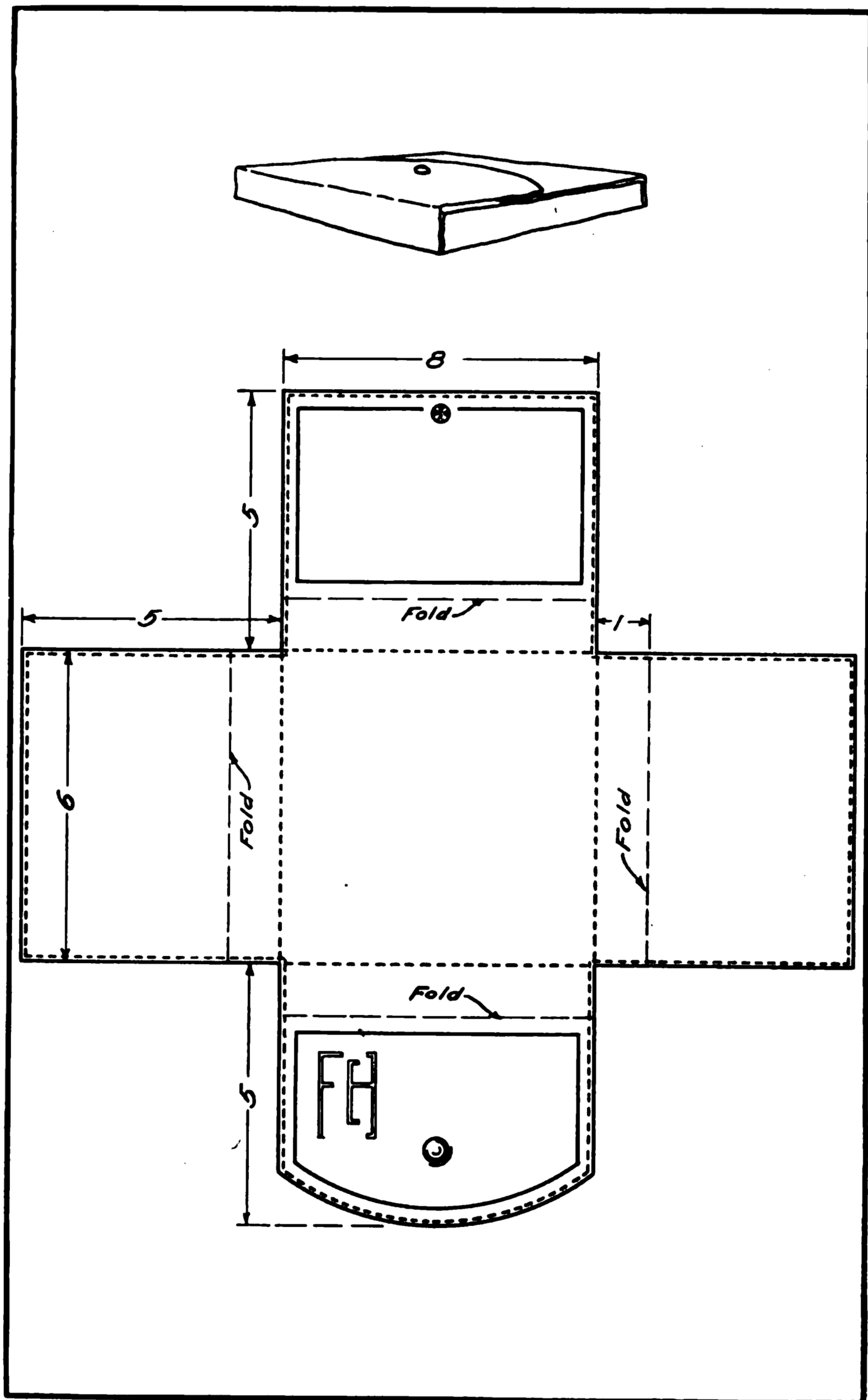
Fig. 27. Gentleman's Handkerchief-Case.
