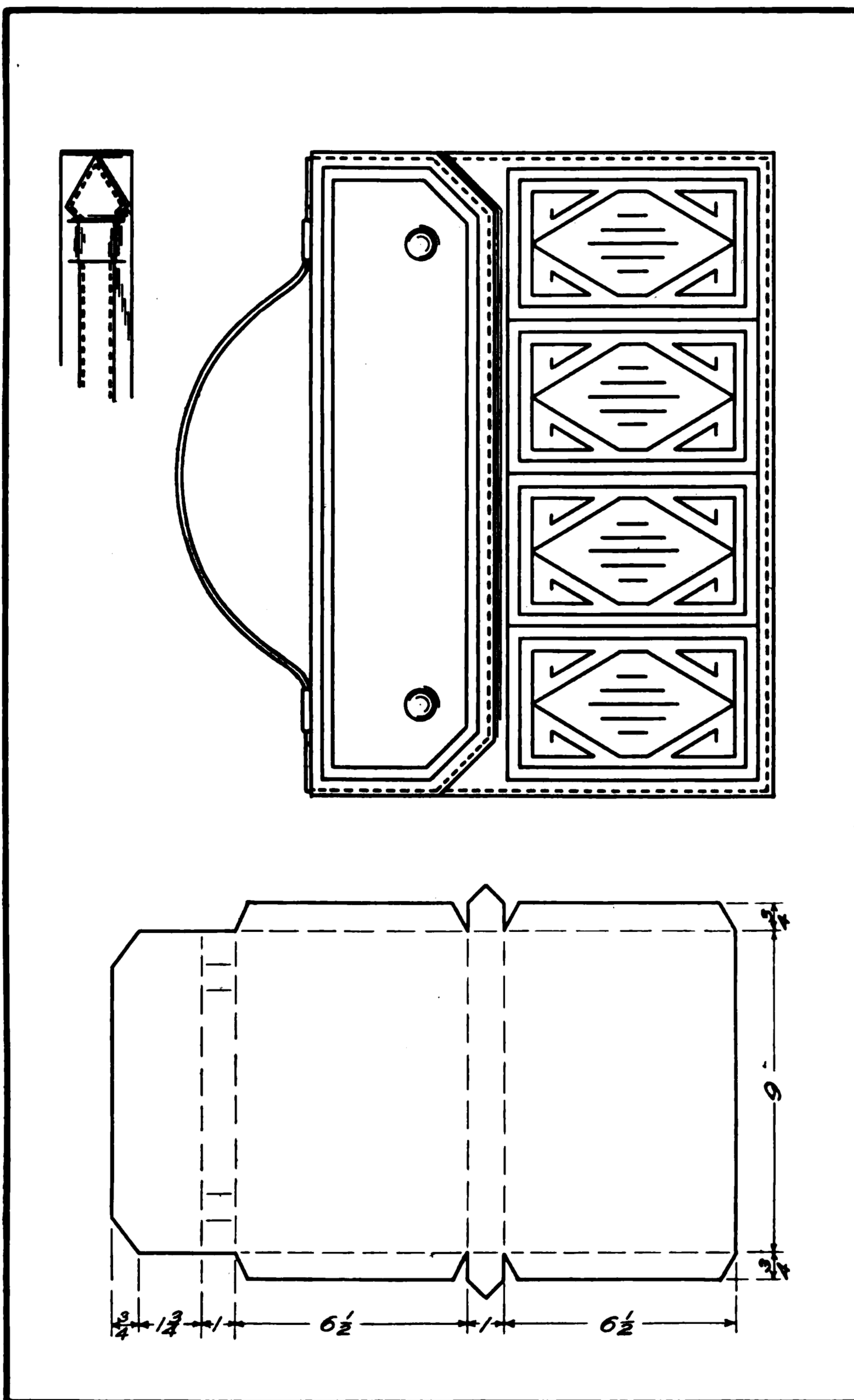
Fig. 28. One-Piece Hand-Bag.
