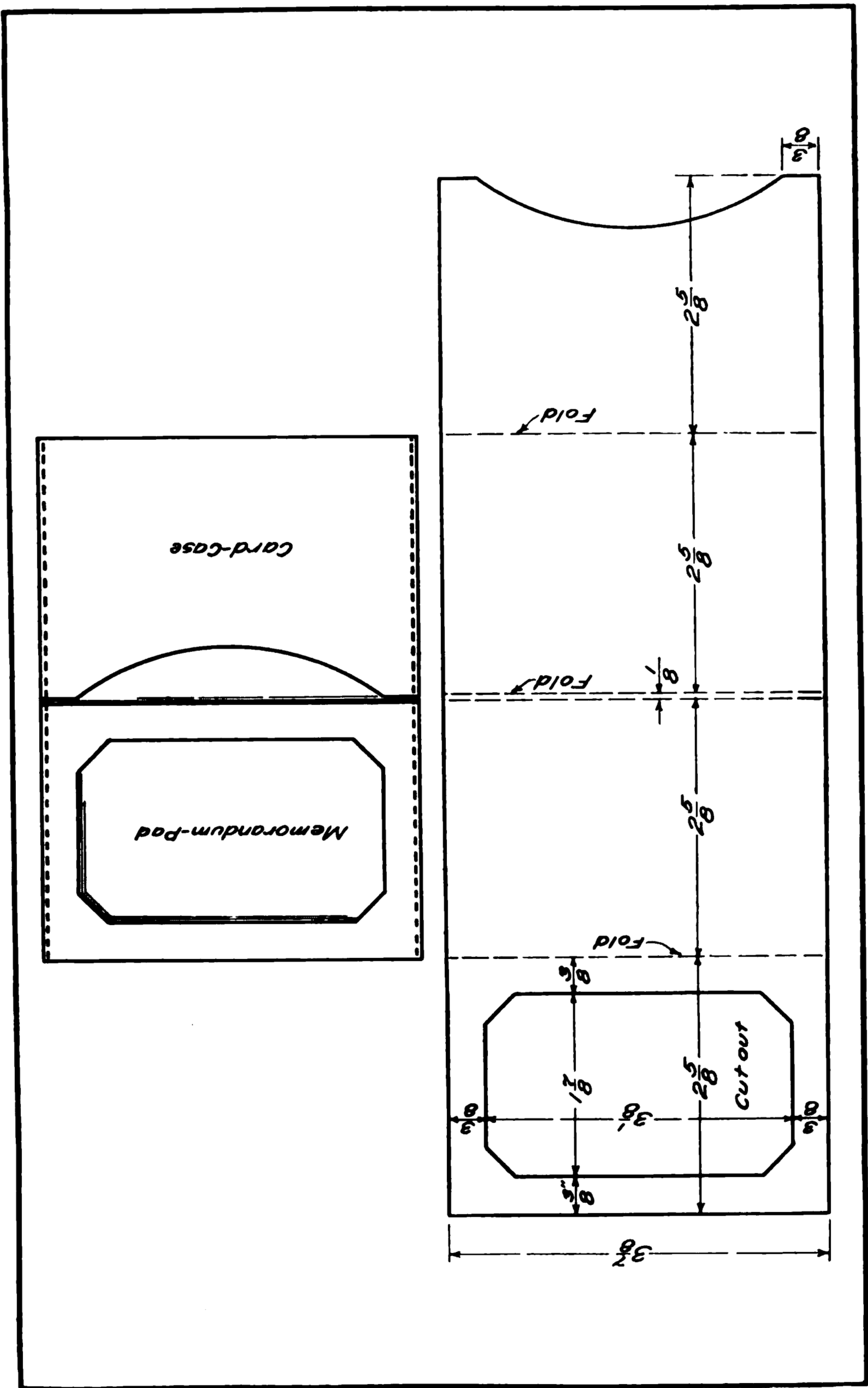
Fig. 38. Folding Memorandum-Pad.
