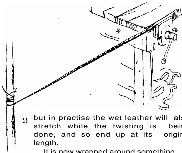
Fig.11. In theory the twisting of the leather should shorten the core,
